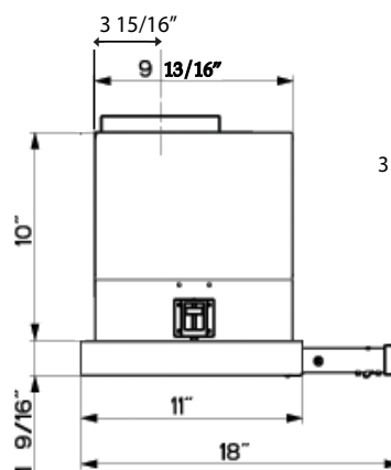
Side View Top Vent
