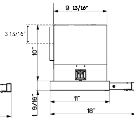
Side Direct Rear Vent
