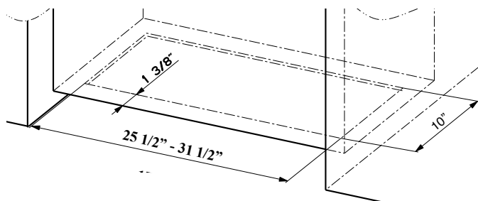
Cabinet Cut Out 30" and 36"
